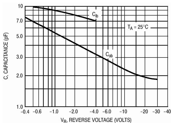
Fig 5. Capacitances
