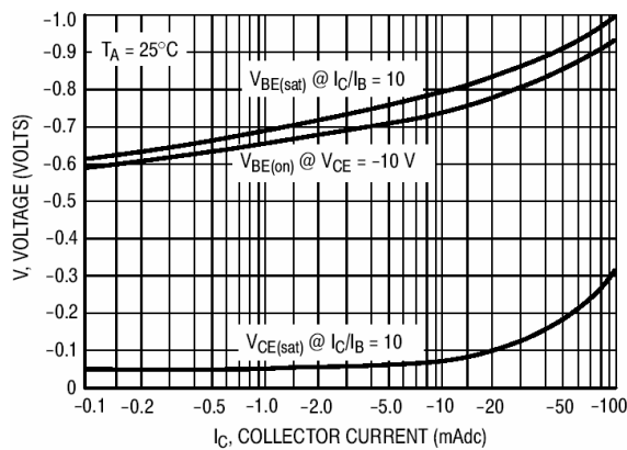
Fig 3. "Saturation" &amp; "On" Voltages
