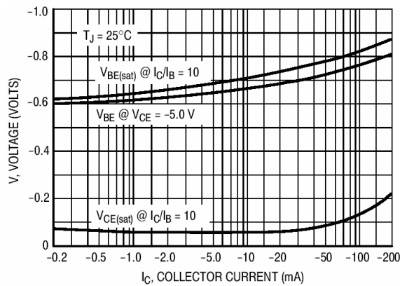
Fig 3. "On" Voltages
