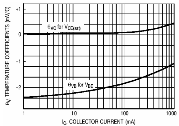
Fig 4. Temperature Coefficients
