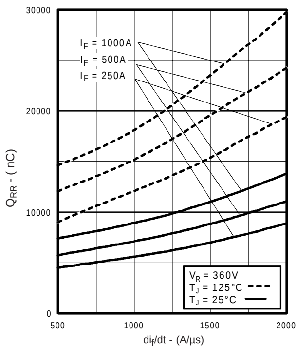
Fig. 14 - Typical Stored Charge vs. di/dt
