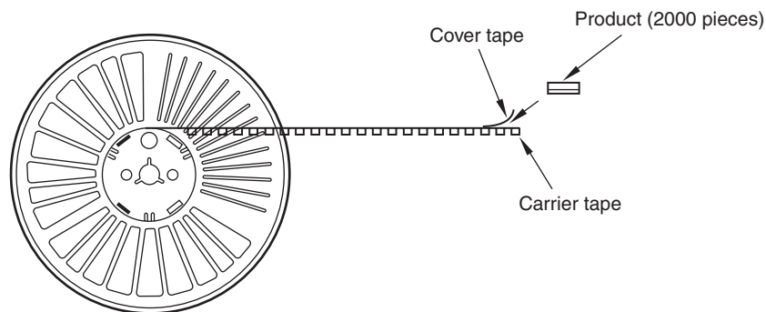
Fig. 5 Inner Packing
