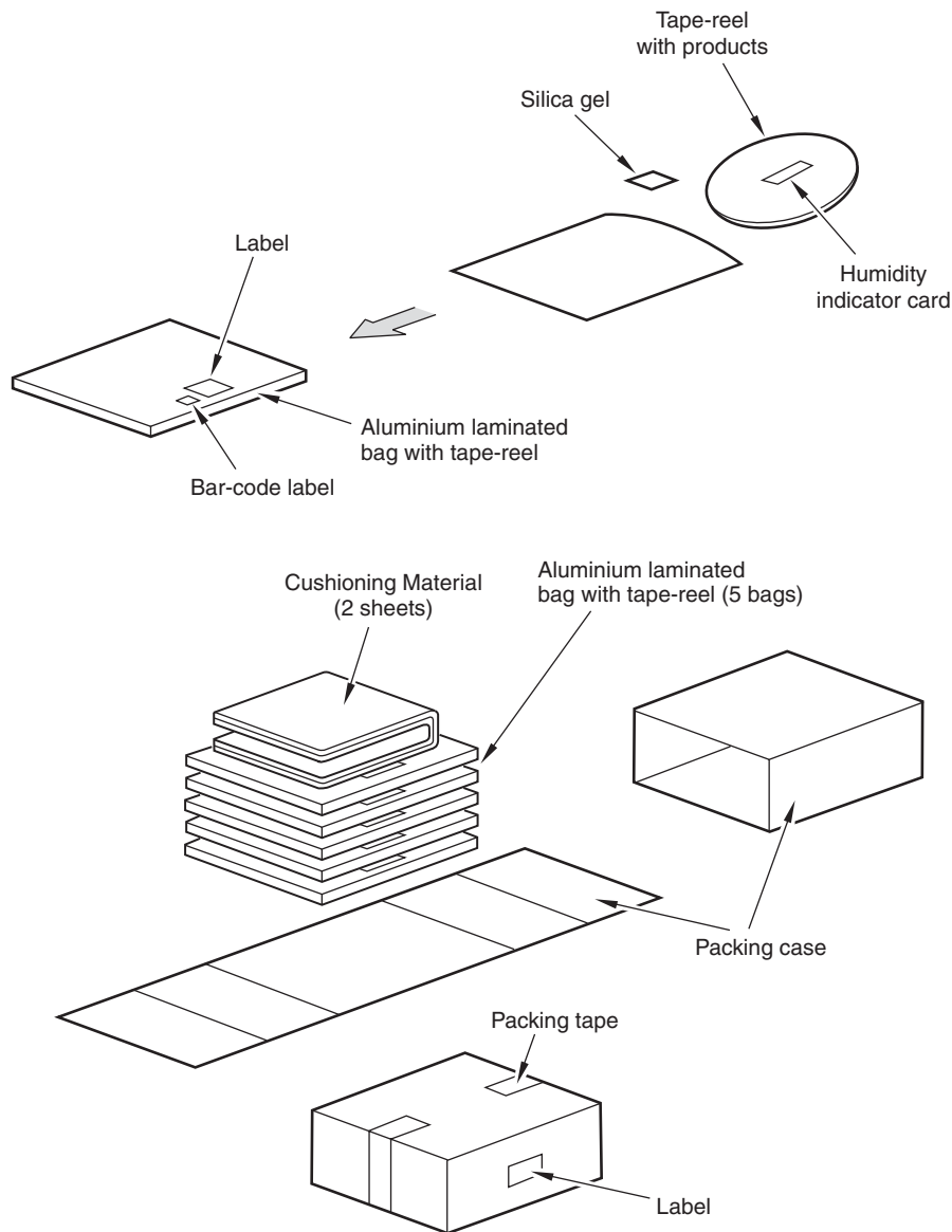
Fig. 6 Packing Specification
