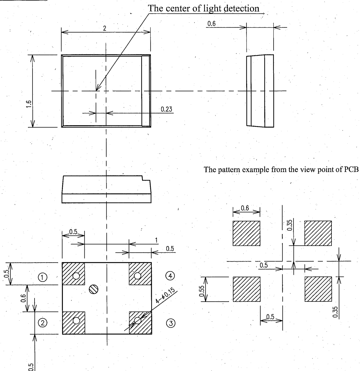
Pin arrangement
