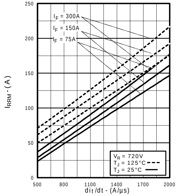
Fig. 16 - Typical Recovery Current vs. di_T/dt
