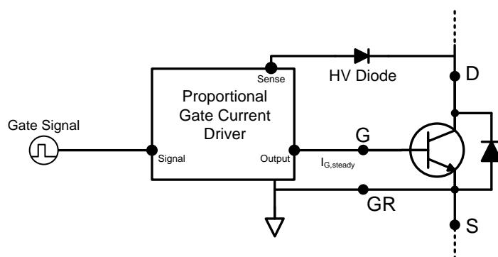
Figure 29: Simplified Voltage Controlled Proportional Driver
