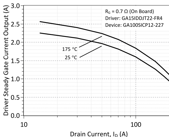
Figure 26: Typical steady state gate current supplied by the GA15IDDJT22-FR4 board for the GA100SICP12-227 with the on board resistance of 0.7 \Omega
