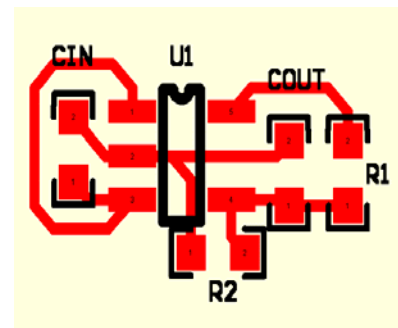
Figure 5. Adjustable Mode
