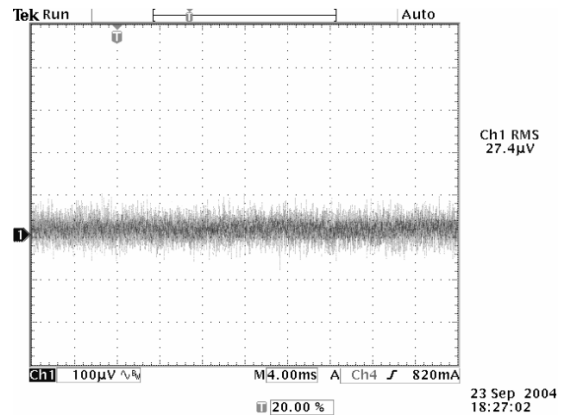
Output Noise
