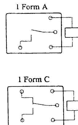
Wiring Diagram
