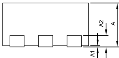
ADFN1.5X1.5-6 Package
