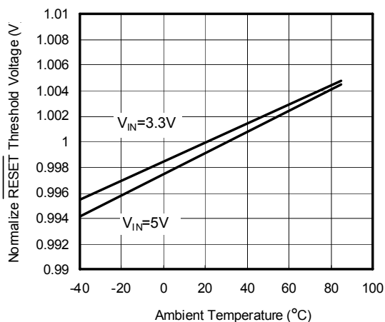
Normalize \overline{\text{RESET}} Threshold Voltage vs. Ambient Temperature
