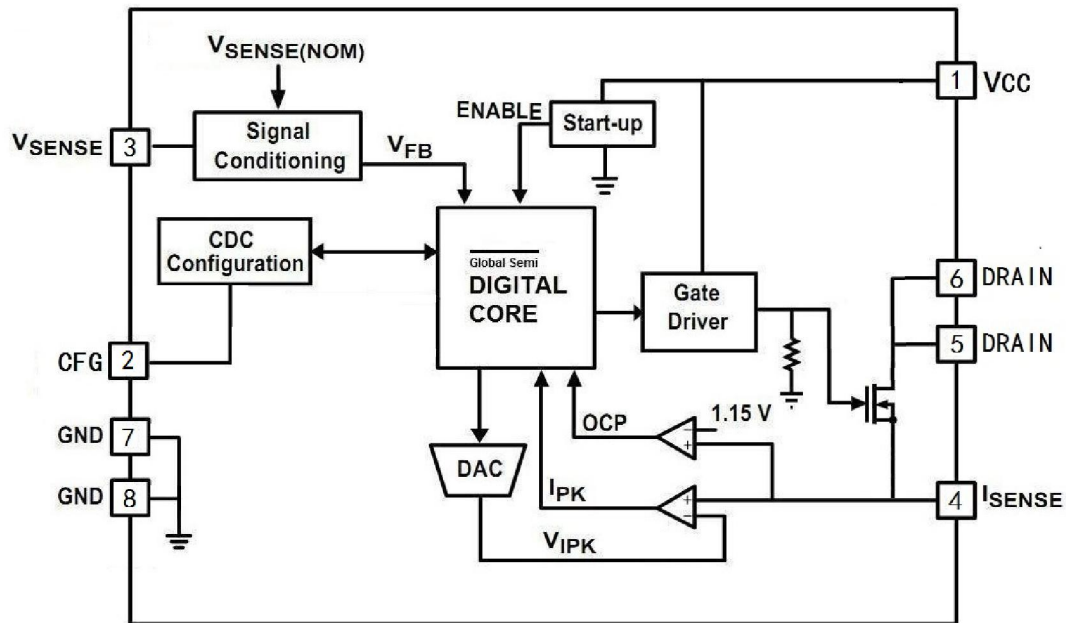
Figure2.1 G5138P Functional Block Diagram
