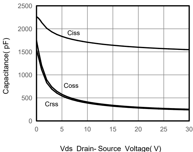
Figure5. Capacitance
