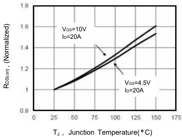
Figure 7. Drain-Source On-Resistance
