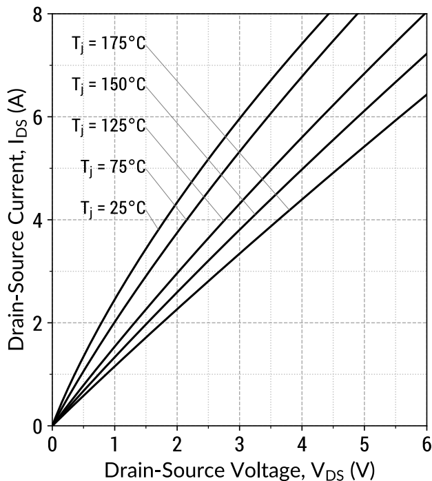
Figure 3: Output Characteristics ( V_{GS} = 15\text{ V} )
