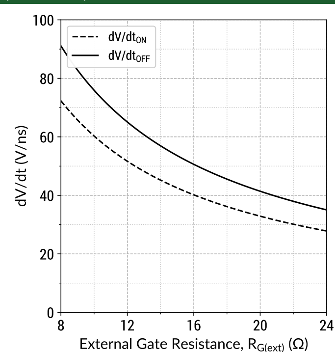
Figure 26: dV/dt v/s R_{G(ext)} ( V_{DD} = 1200V )
