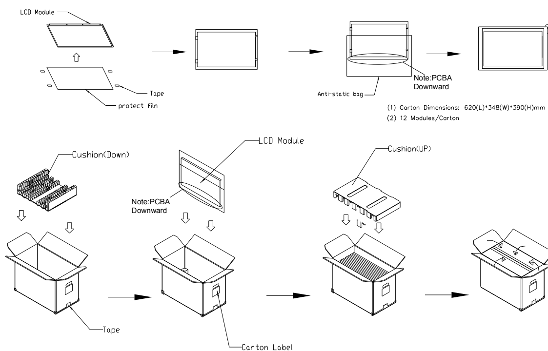
Figure. 7-1 Packing method
