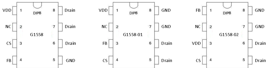
Pin Configuration: G1558 Series
