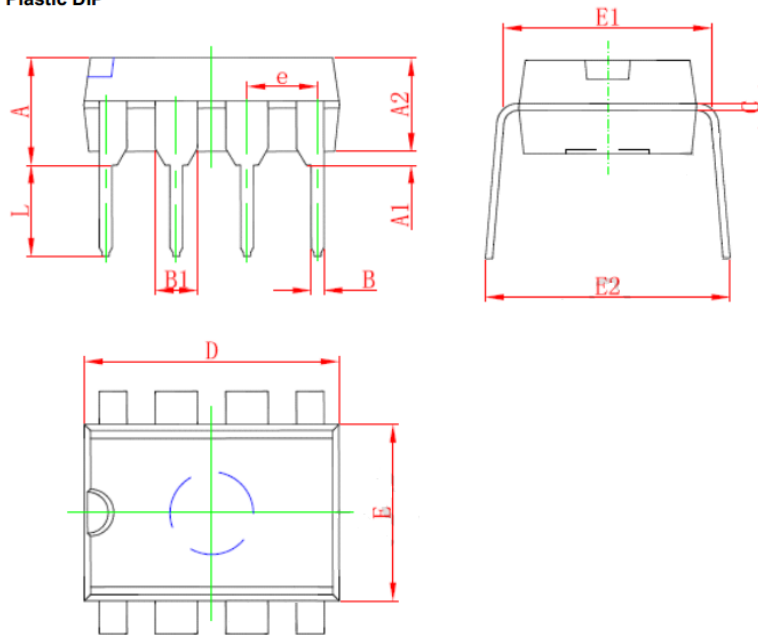
8-Pin Plastic DIP
