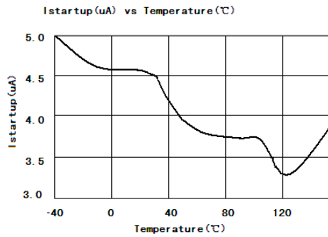
Figure 6.1 Istartup(uA) vs Temperature(°C)
