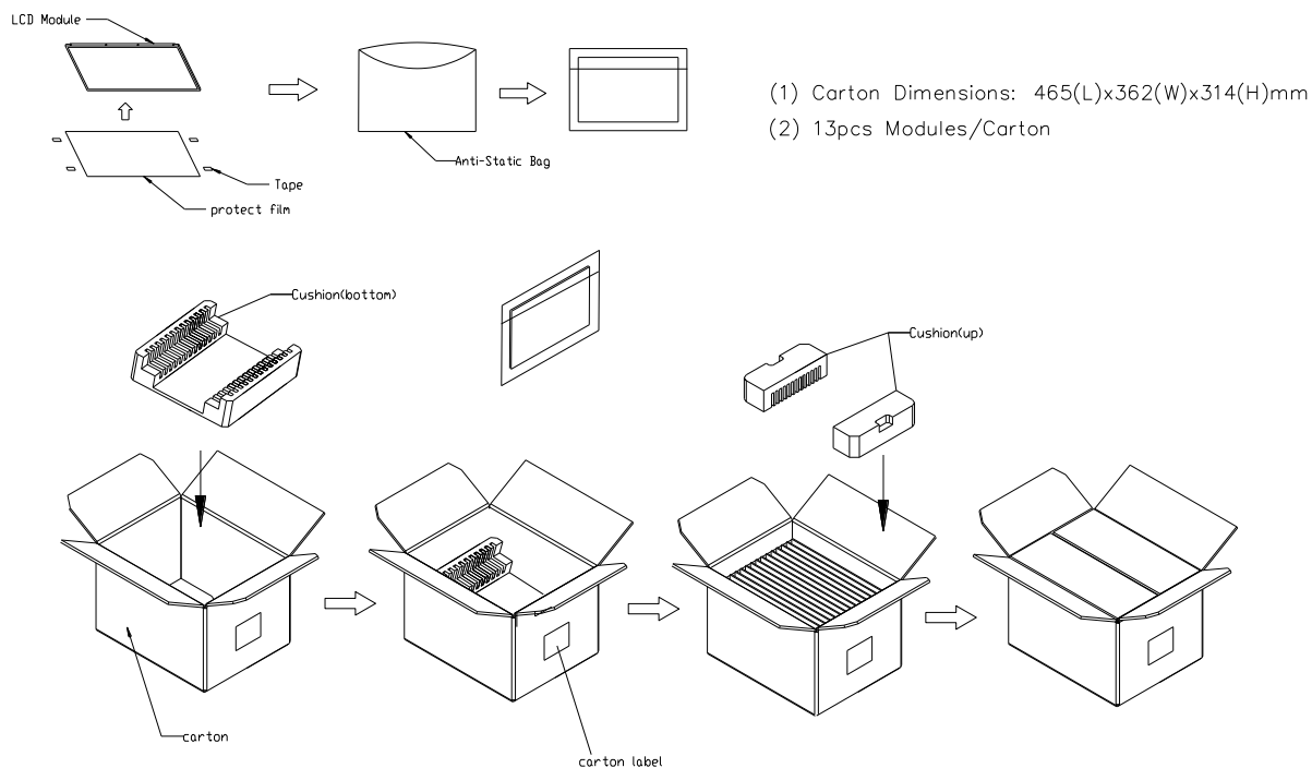
Figure. 9-1 Packing method
