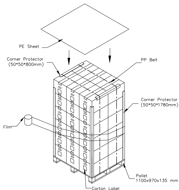
Figure. 9-2 Packing method
