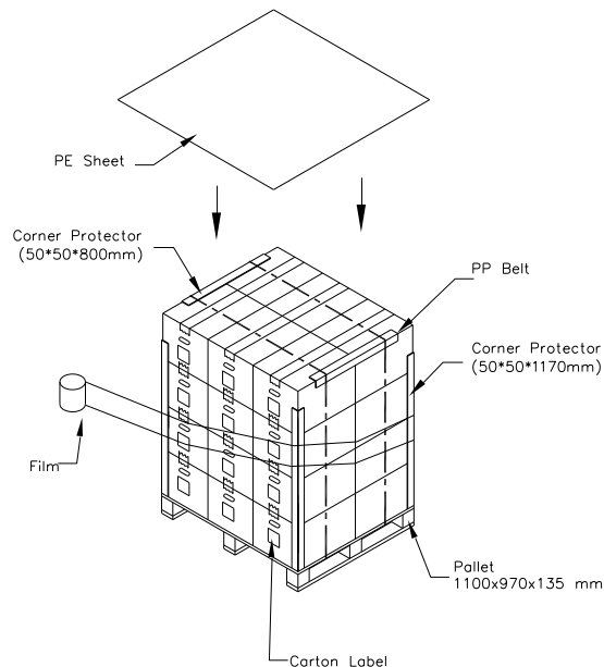
Figure. 9-2 Packing method
