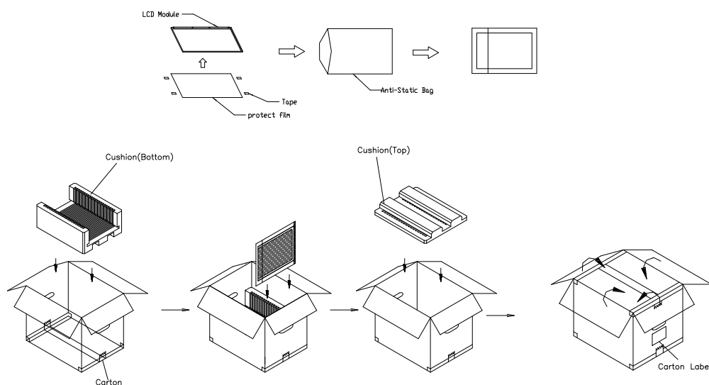
Figure. 6-1 Packing method
