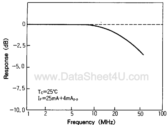
Frequency response
