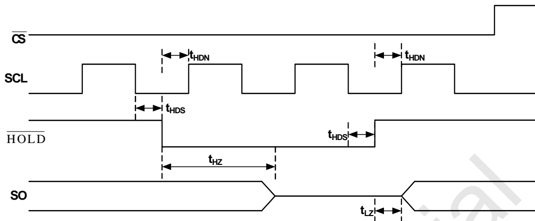
Figure 3: HOLD Timing
