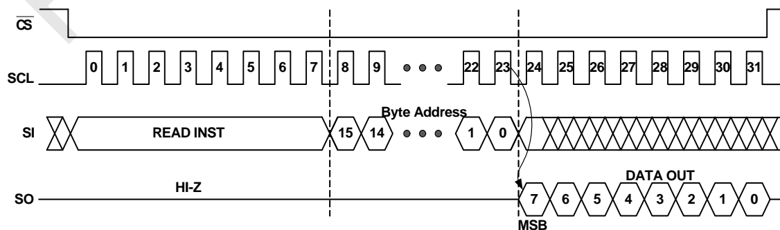
Figure 9: READ Timing
