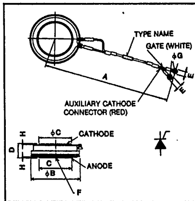
FT2500CL Outline Drawing
