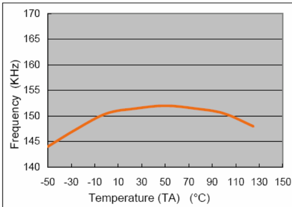
FSP3125 Frequency v.s. Temperature (Vcc=12V , Io=500mA , Vout=5V)
