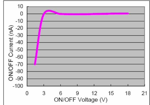
FSP3125 ON/OFF Current v.s. ON/OFF Voltage (Vin=12V)
