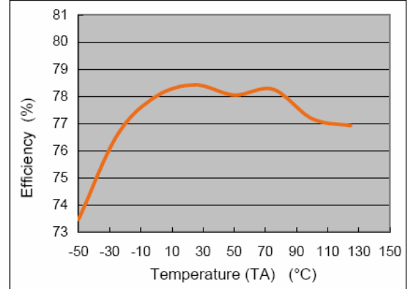
FSP3125 Efficiency v.s. Temperature (Vin=12V,Vout=3.3V,Io=2A)
