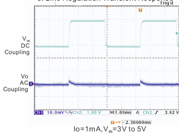
8. Line Regulation Transient Response
