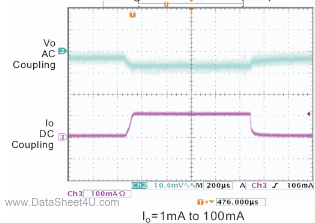
7. Load Regulation Transient Response
