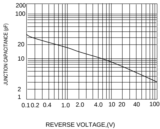
Figure 4 TYPICAL CAPACITANCE
