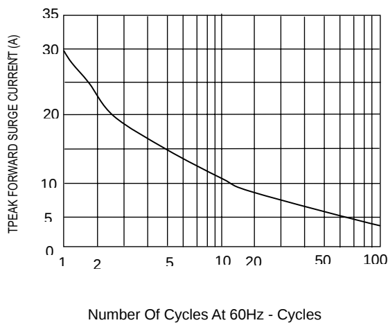
Figure 3 NON-REPETITIVE FORWARD SURGE CURRENT
