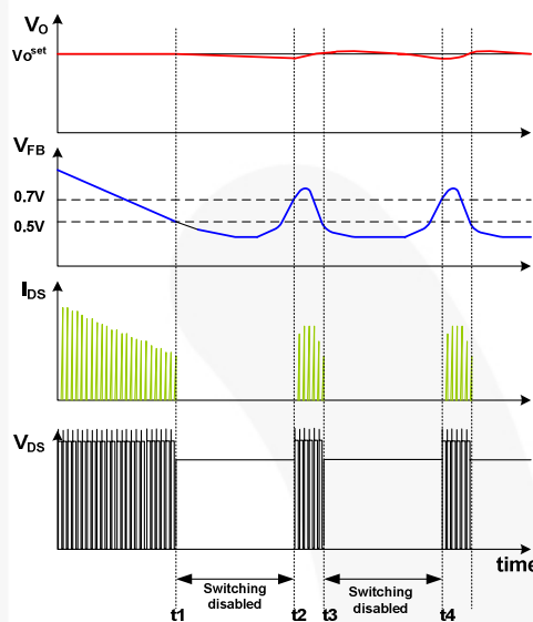
Figure 22. Burst-Mode Operation
