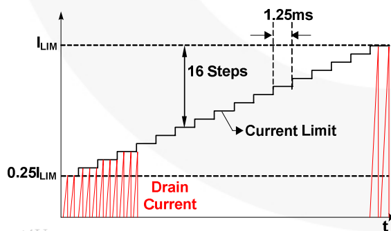
Figure 21. Internal Soft-Start
