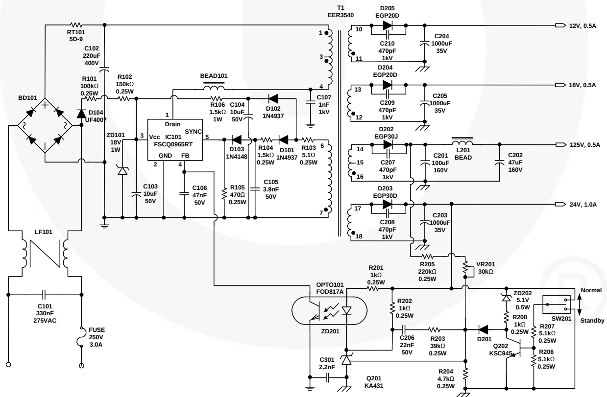
Figure 43. FSCQ0965RT Typical Application Circuit Schematic
