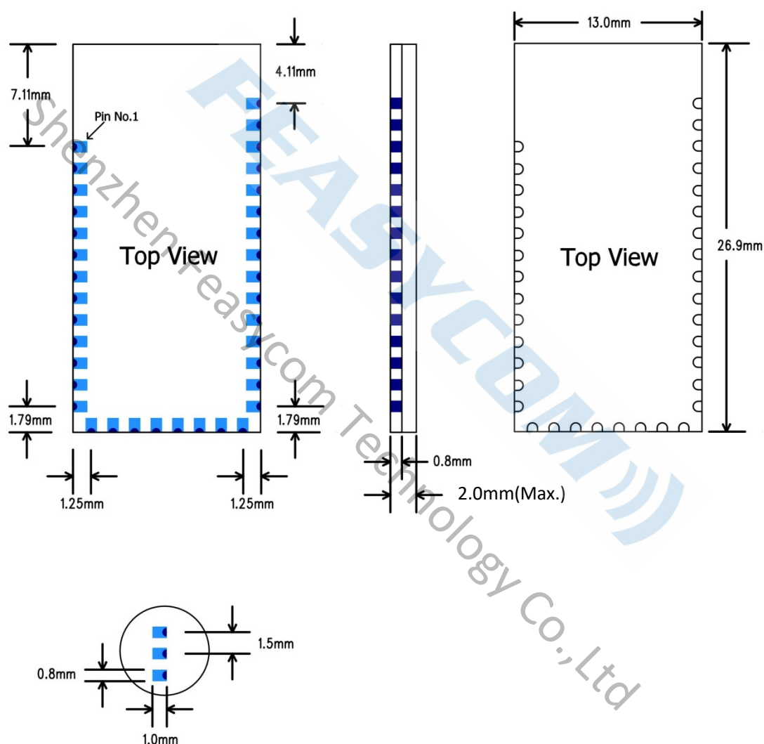
Figure 7: FSC-BT946 footprint
