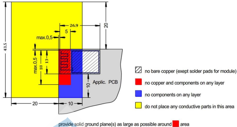
Figure 6: FSC-BT836B Restricted Area
