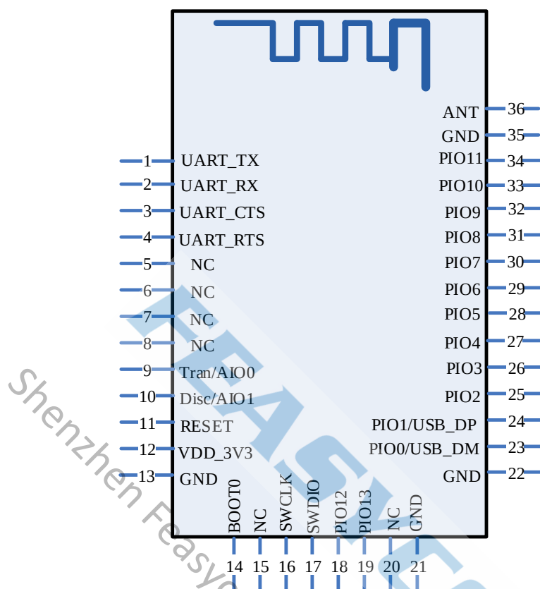
Figure 1: FSC-BT836B PIN Diagram
