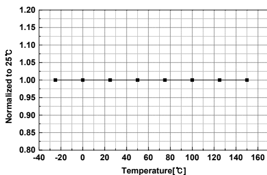
Figure 4. Stop Threshold Voltage vs. Temp.
