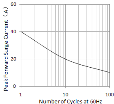
Figure 2. Maximum Non-Repetitive Peak Forward Surge Current
