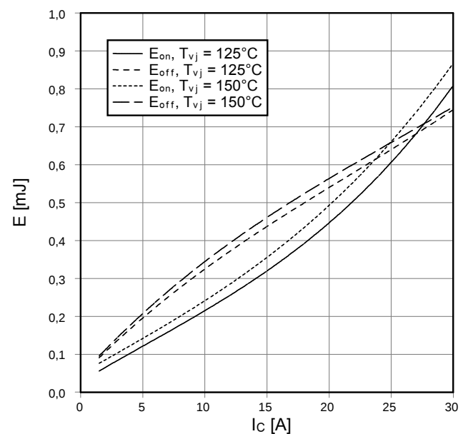
Schaltverluste IGBT-Wechselr. (typisch) switching losses IGBT-inverter (typical) E_{on} = f(I_C) , E_{off} = f(I_C) V_{GE} = \pm 15\text{ V} , R_{Gon} = 22\ \Omega , R_{Goff} = 22\ \Omega , V_{CE} = 300\text{ V}
