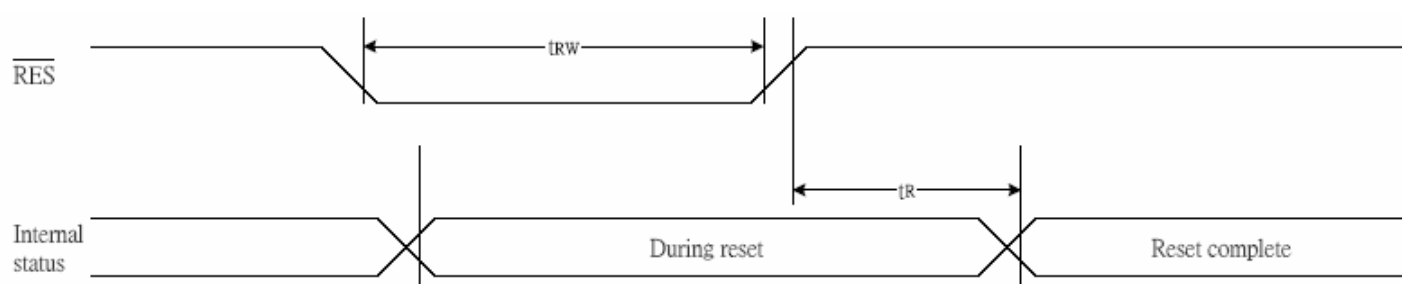
Figure 5: Reset Timing
