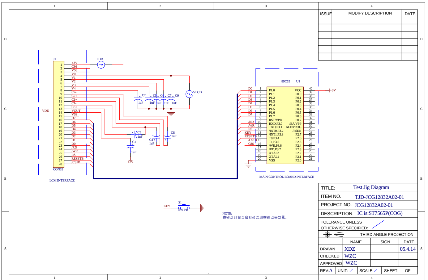
Figure 2: Recommend the outer circuit
