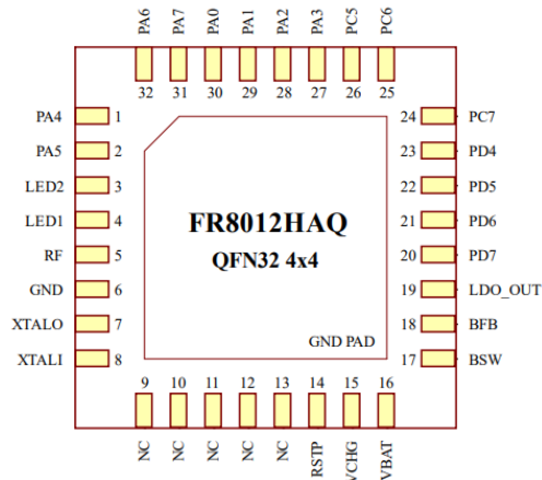
Figure 2-1 FR8012HAQ pin information
