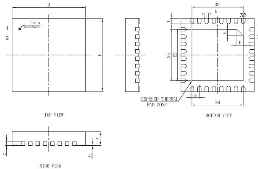
Figure 2-2 Package Physical Dimensions
