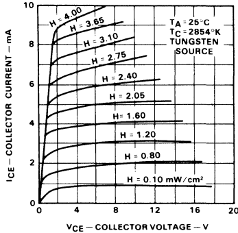
FPT120/A/B/C Collector Current vs Collector Voltage
