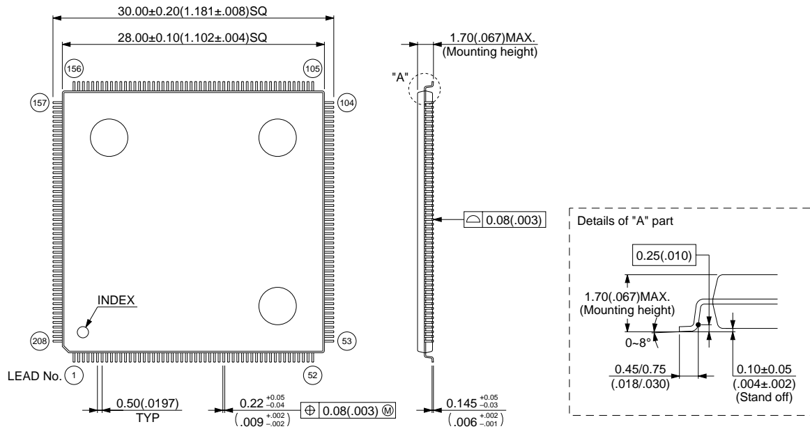
208-pin plastic LQFP (FPT-208P-M06)
