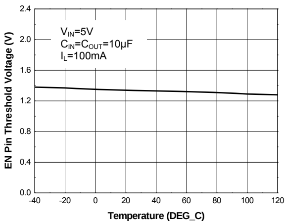
Figure 13.EN Pin Threshold Voltage vs. Temperature
