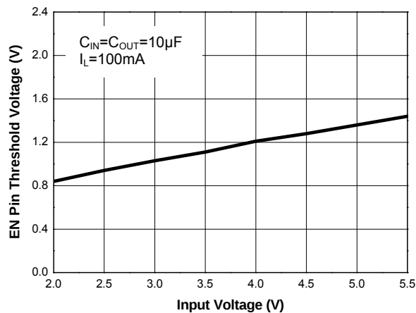
Figure 12.EN Pin Threshold Voltage vs. Input Voltage
