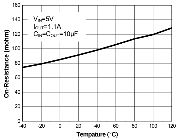
Figure 10. On-Resistance vs. Temperature
