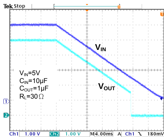
Figure 22. UVLO at Falling
