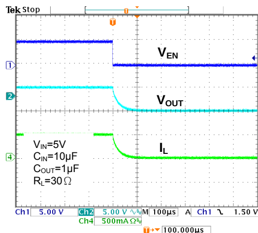
Figure 20. Turn-off Response
