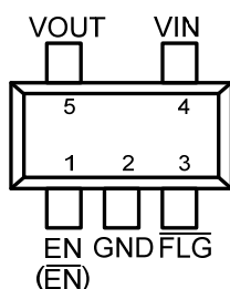
Figure 1. Pin Assignment of FP6861
