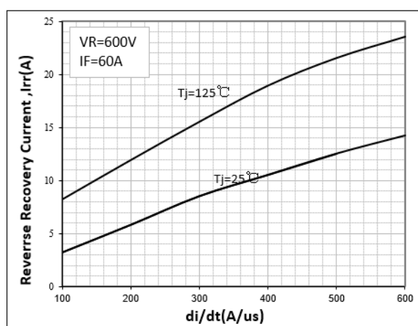
Fig.4 Reverse Recovery Current vs dI_F/dt
