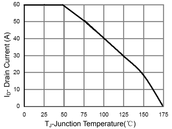
Figure 9 ID De-rating
