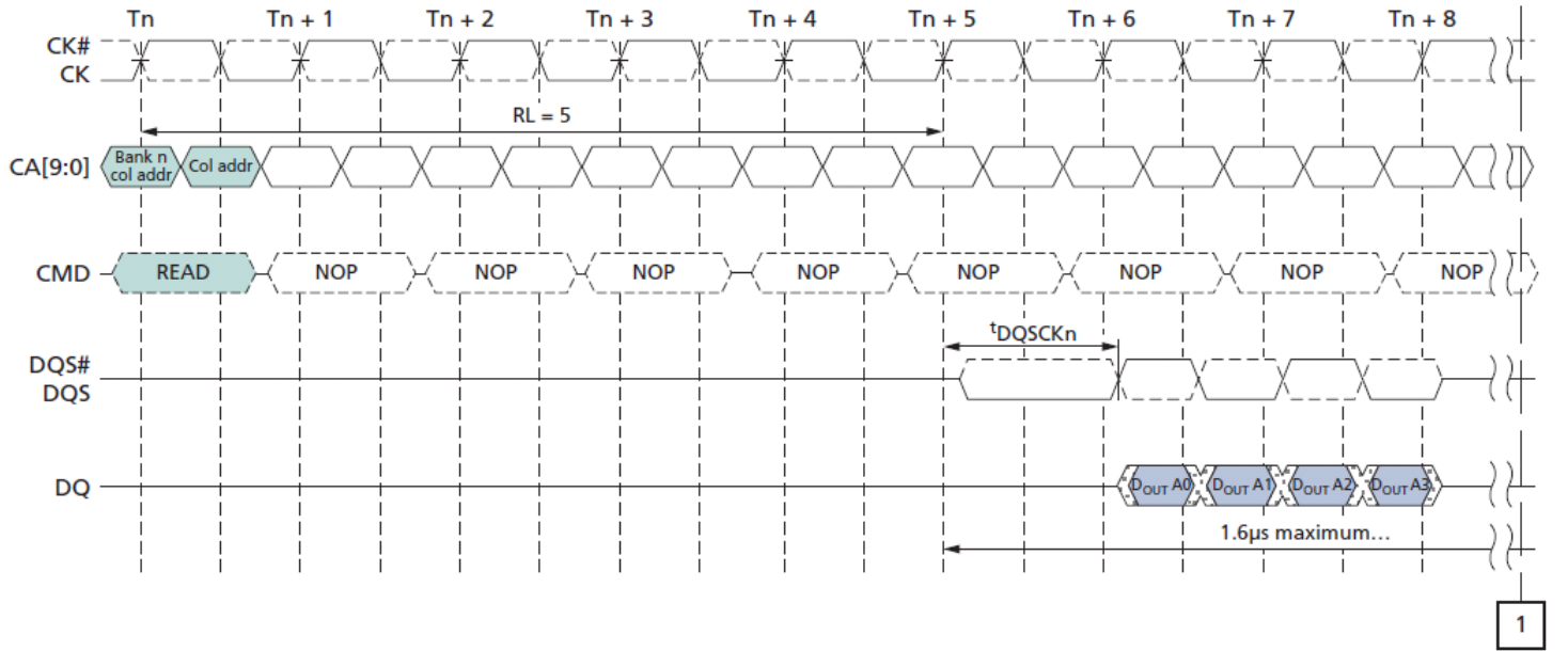
Figure 9 : tDQSKDM Timing
