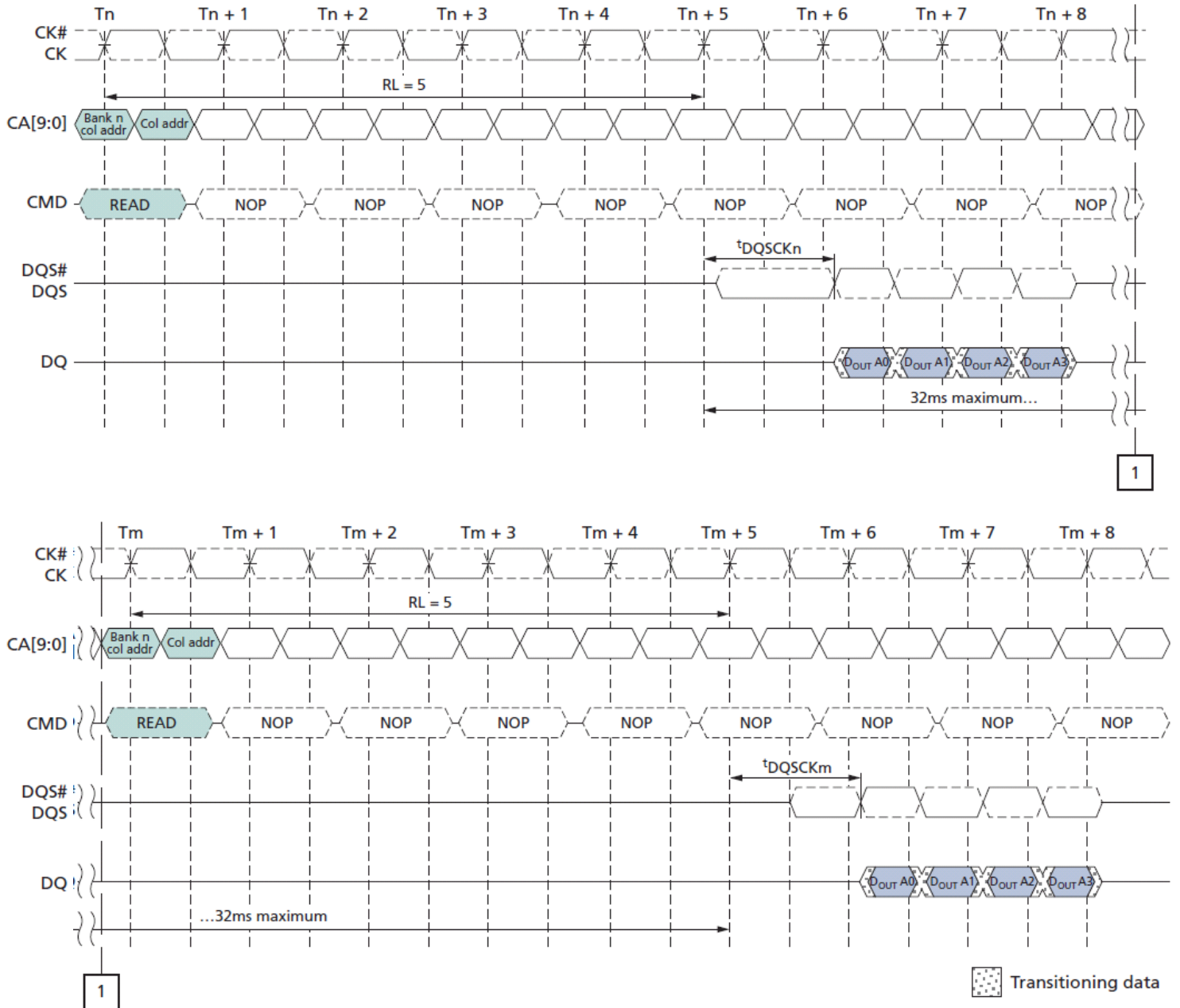
Figure 8 : tDQSKDL Timing
