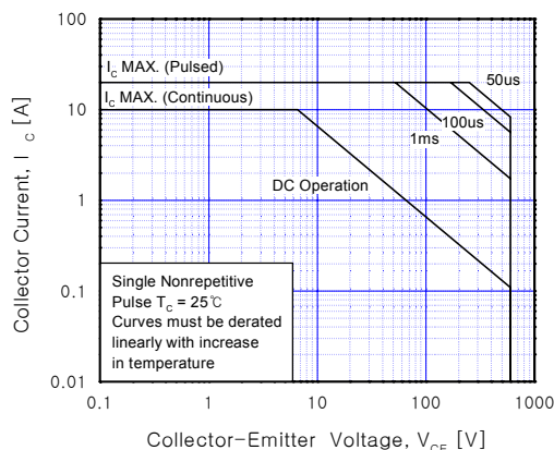
Figure 15. SOA Characteristics
