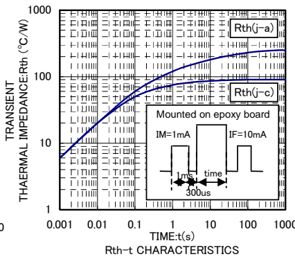
Rth-t CHARACTERISTICS
