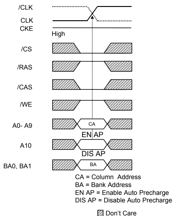
Figure 6: READ Command
