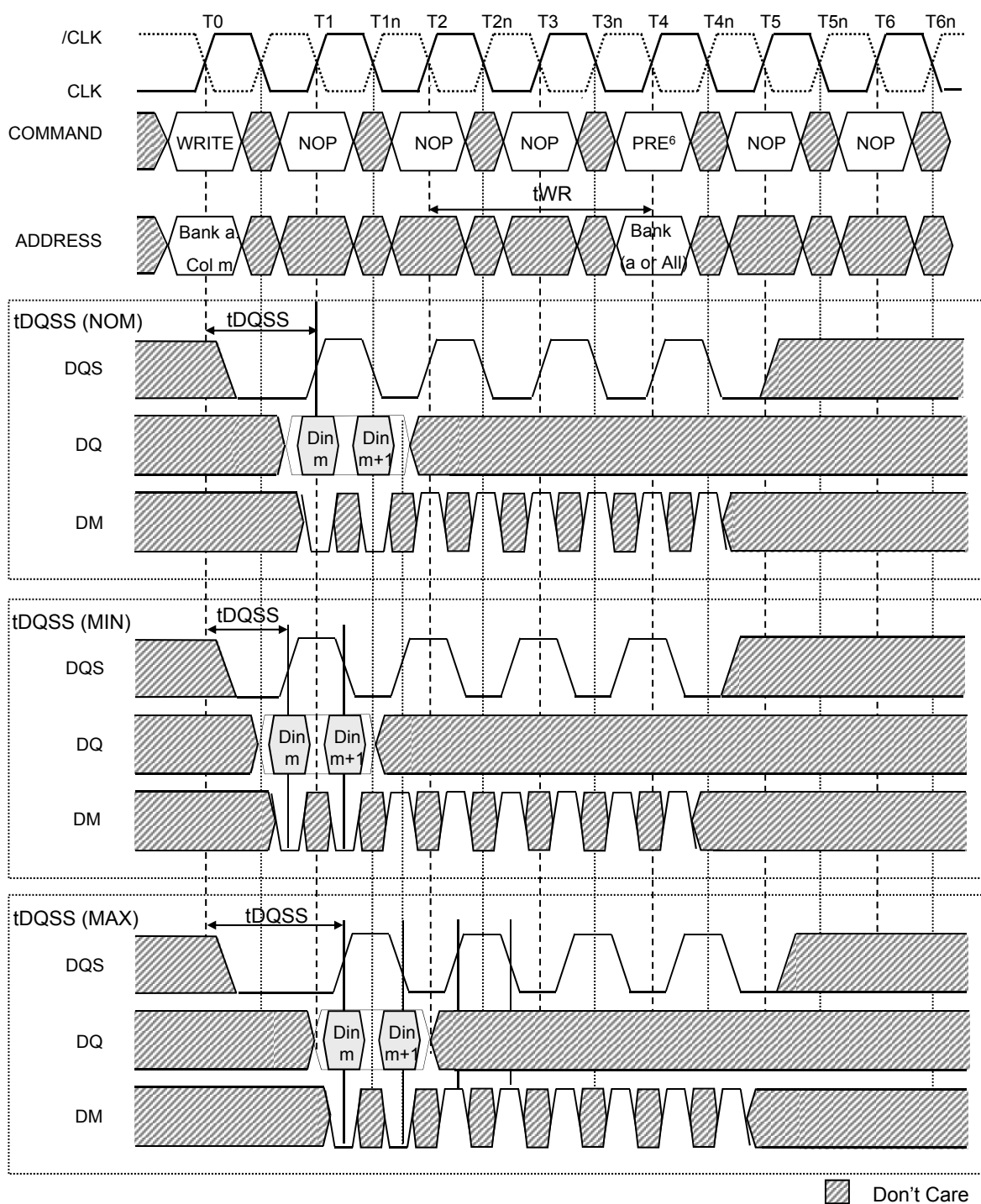
Figure 23: WRITE-to-PRECHARGE – Interrupting
