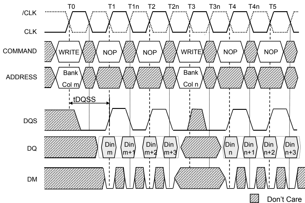
Figure 17: WRITE-to-WRITE Operation
