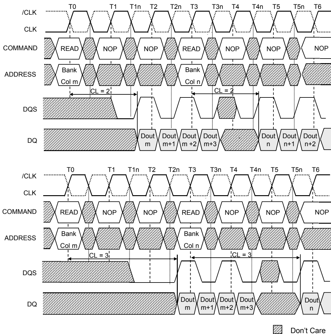
Figure 9: Read-to-Read Operation
