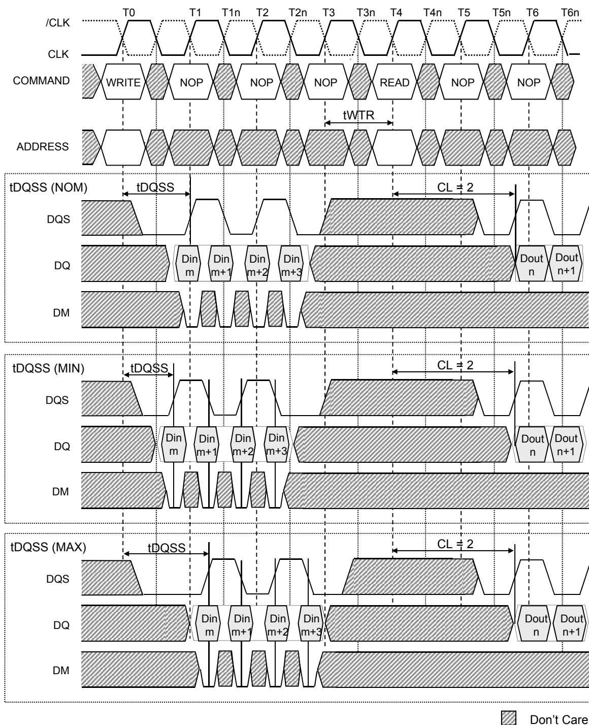
Figure 19: WRITE-to-READ – Uninterrupting
