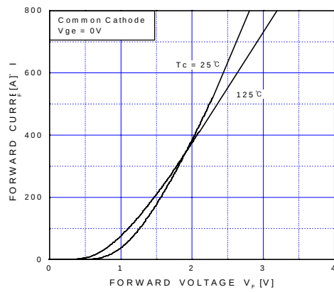
Fig 19. Forward Characteristics
