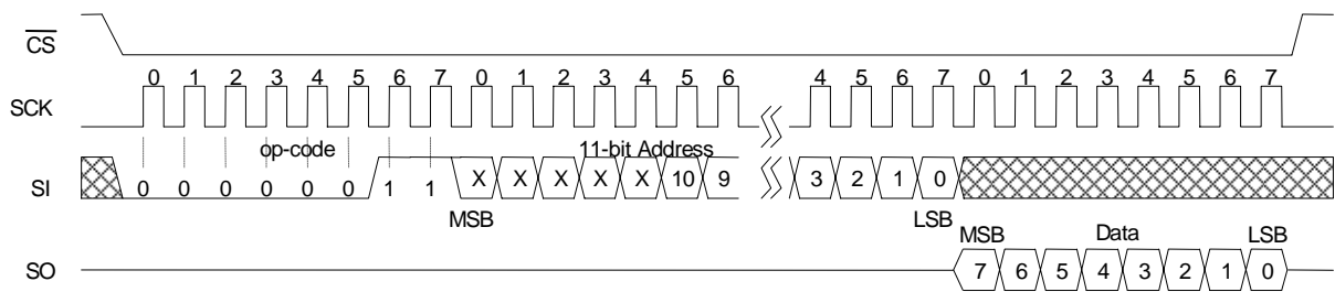
Figure 10. Memory Read
