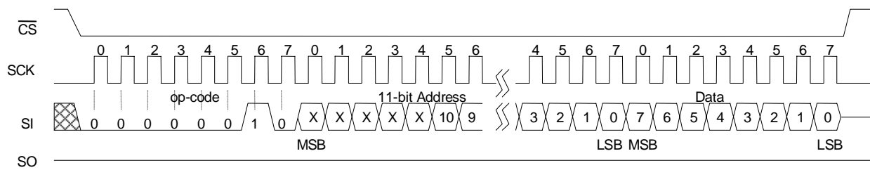
Figure 9. Memory Write
