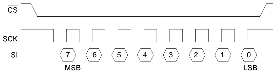
Figure 4. SPI Modes 0 & 3
