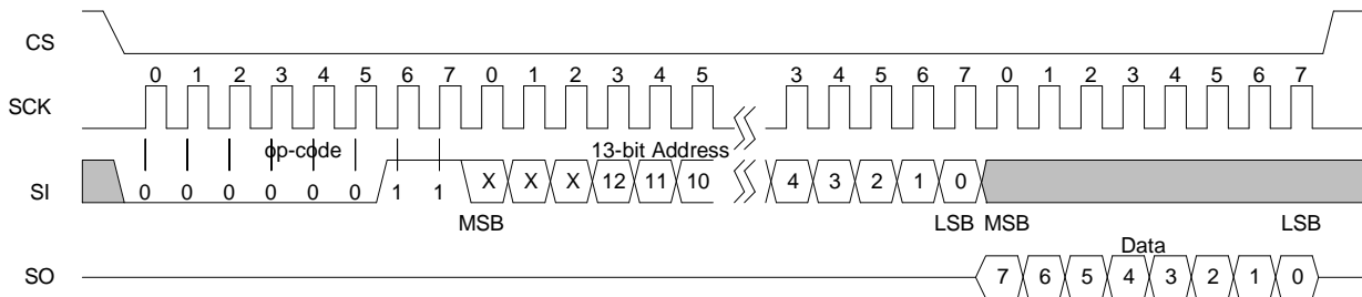
Figure 10. Memory Read
