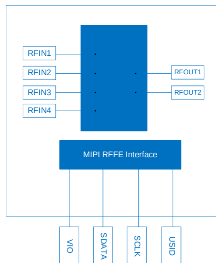
Figure 1 Functional Block Diagram and Pin Configuration
