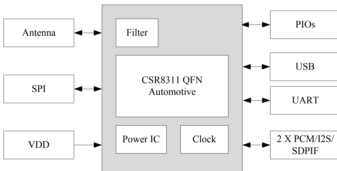
Figure 1: Block Diagram
