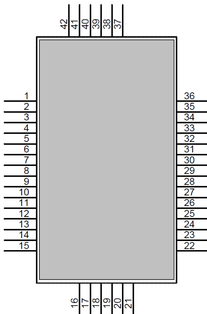
Figure 2: Pin Configuration
