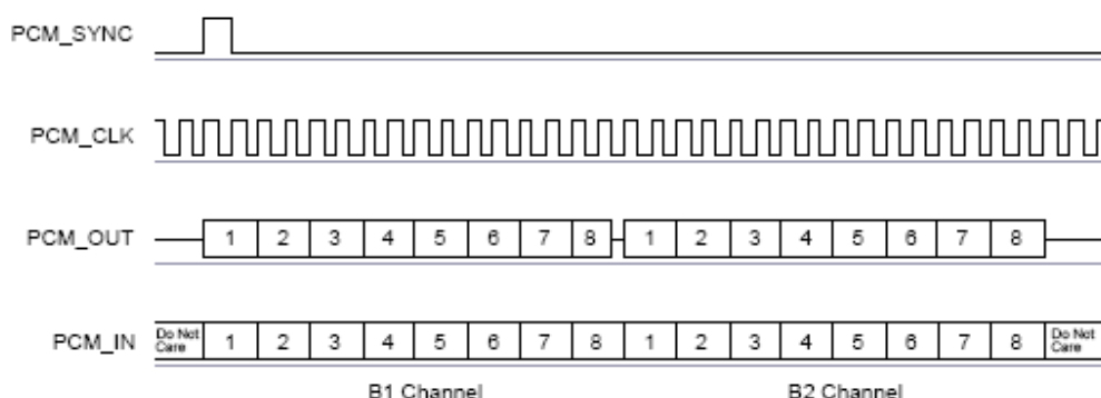
Figure 8: GCI Interface
