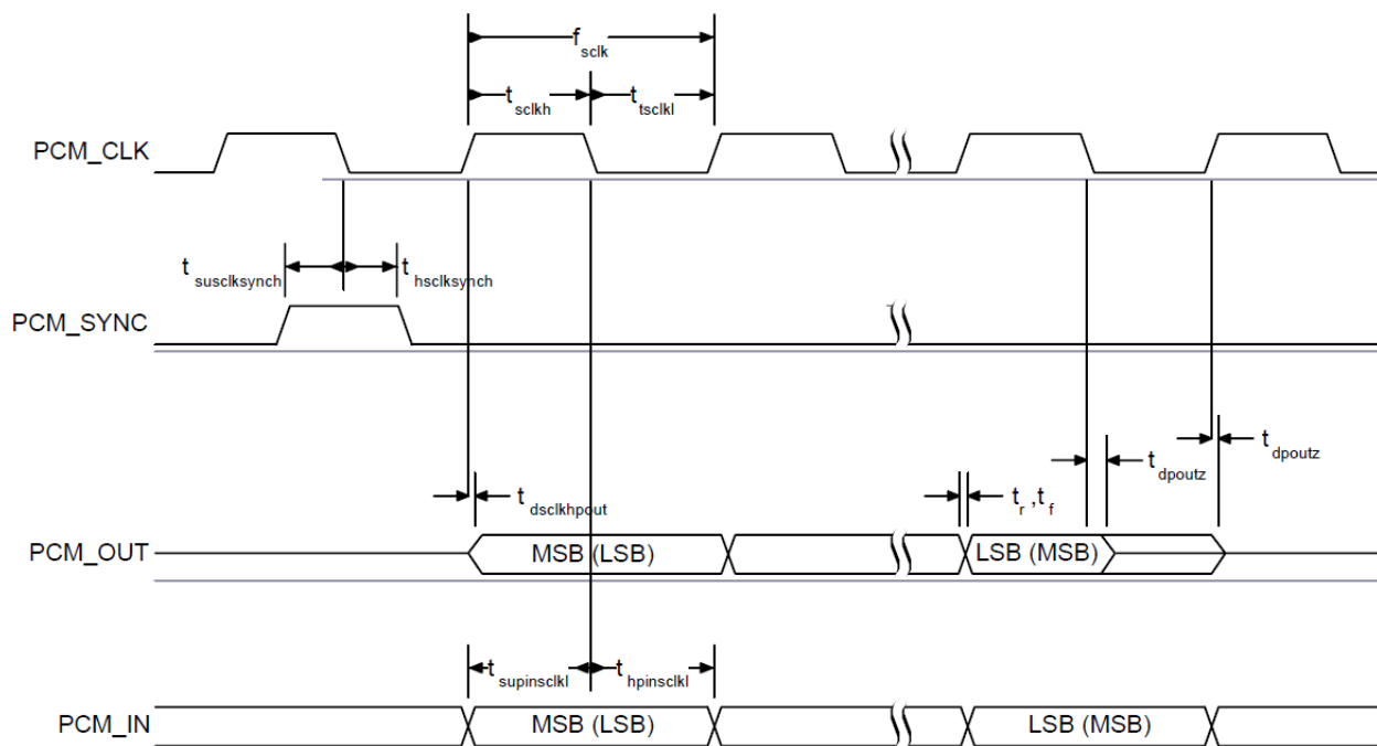
Figure 13: PCM Slave Timing Short Frame Sync
