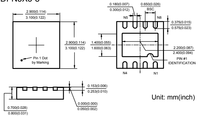
DFN3X3-8
