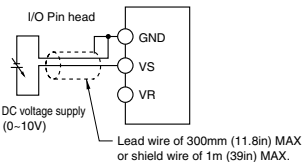
Fig.2 Speed setting by external voltage supply
