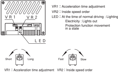
Fig3 Driver external from and internal organs LED and a trimmer
